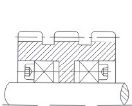
大齿轮的两边用胀套受力均匀 Equally under stress on two sides of large gear by locking device
