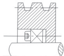
单只Z2型胀套与轴连结 Connection of single Z2 type locking device with axle
