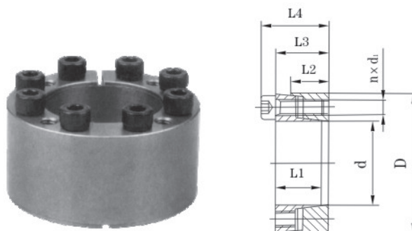
图十五 Z 15 型胀紧联结套 Drawing15 Z 15 Type Locking Device
