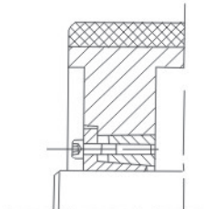
胀套用于皮带输送机传动滚筒中，改善焊接性，便于装拆 Locking device applied in transmission cylinder of belt conveyer can improve weldability and easy for disassemble.
