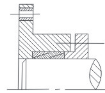
精密传动正反转无键带来的间隙 The accurate transmission is transferred positive and negatively to the interval that without key to bring
