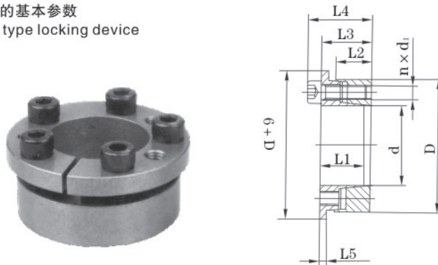
图十六 Z 16 型胀紧联结套 Drawing16 Z 16 Type Locking Device
