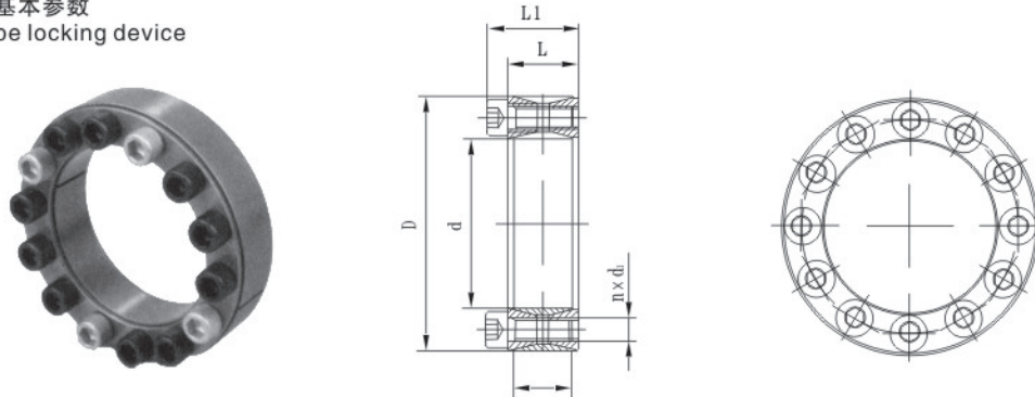
图二 Z 2 型胀紧联结套 Drawing 2 Z 2 type Locking device
