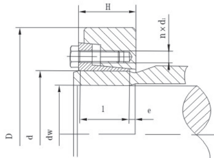
图十 Z 10 型胀紧联结套 Drawing 10 Z 10 Type Locking Device
